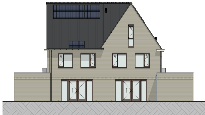
T25, T38, T49 T24, T39, T48 achtergevel (1:100)
