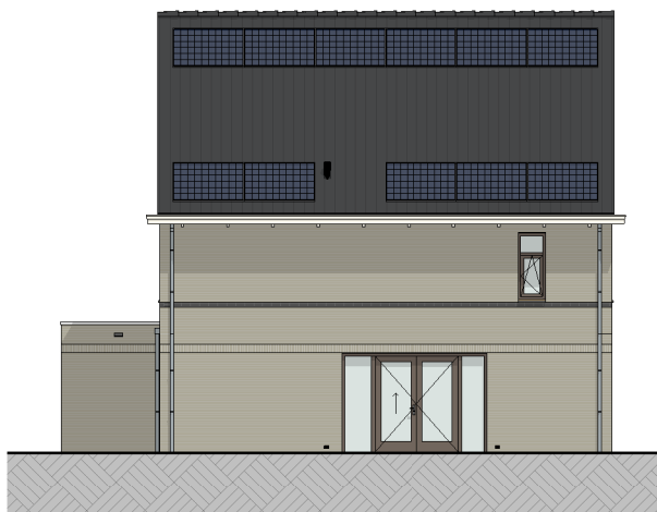
V46 linkergevel (1:100)
