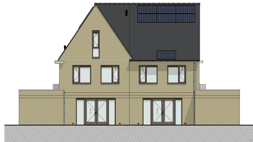
T31, T53 T30, T52 achtergevel (1:100)
