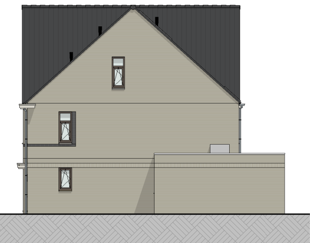
T25, T38, T49 rechtergevel (1:100)
