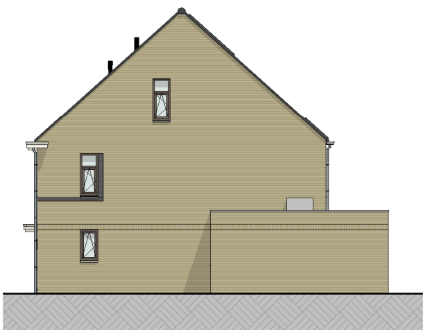
T27, T29, T42, T51 rechtergevel (1:100)
