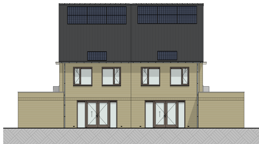
T27, T29, T42, T51 T26, T28, T43, T50 achtergevel (1:100)
