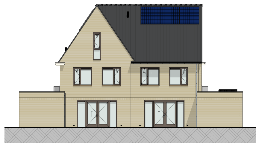
T44 T45 achtergevel (1:100)
