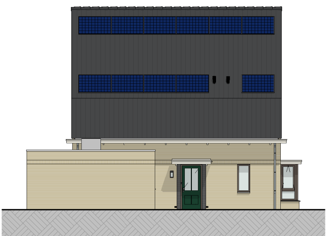
V33, V36 linkergevel (1:100)
